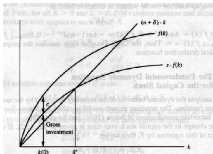
Graph 1.1 - Solow-Swan model
